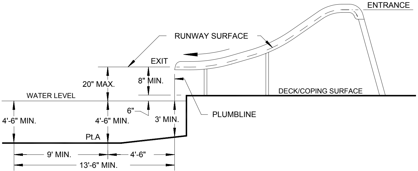
CRITICAL DIMENSIONS FOR SLIDE PLACEMENT
