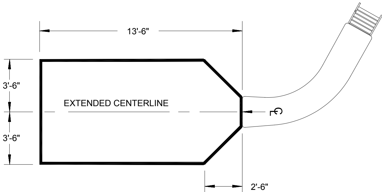
SLIDE MINIMUM CLEARANCE AREA
